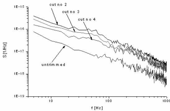
Fig. 12. Power spectral density of “excess” low frequency noise for untrimmed and laser trimmed three-terminal with rectangle additional contact (down) 2×1 mm 2 DP 2041 resistors
