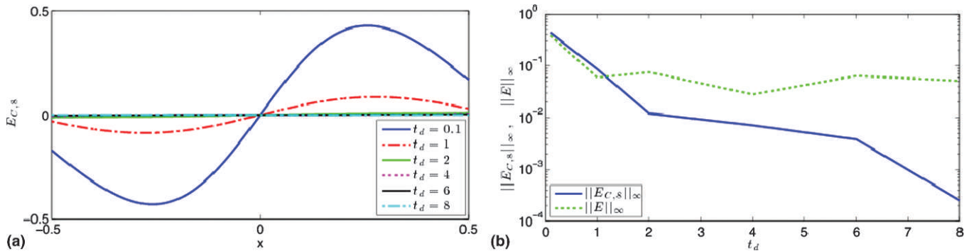
Fig. 15. (a) Error E_{C,s} as t_d varies from 0.1 to 8 in the delayed Gaussian example with N = 1001 , b = 0.096 . (b) \|E_{C,s}\|_\infty as a function of t_d compared with \|E\|_\infty (without continuation).
