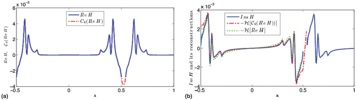
Fig. 8. (a) \text{Re}H(x) and its periodic 8th degree polynomial continuation C_8(\text{Re}H(x)) in the example of a finite element model of a DRAM package with N = 11 , b = 0.0202 shown on [-0.5, 1] . (b) \text{Im}H(x) superimposed with H[C_8(\text{Re}H(x))] and H[\text{Re}H(x)] .
