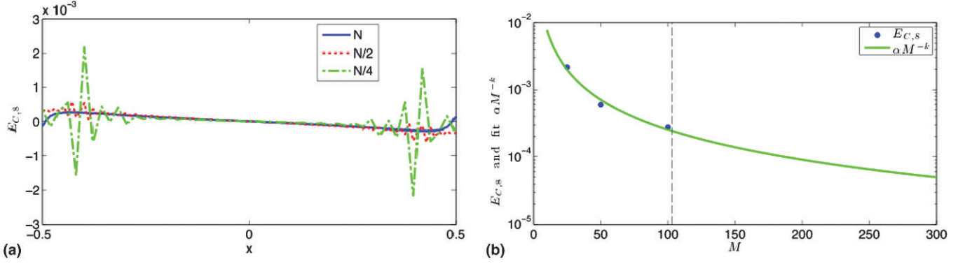
Fig. 10. (a) Errors E_{C,s} of approximation of \text{Im}H(x) by -H[C_8(\text{Re}H)] in the example of a finite element model of a DRAM package with N , N/2 , and N/4 , where N = 100 was used to estimate the smoothness k of the continuation. (b) Norms of the reconstruction errors \|E_{C,s}\|_{\infty} with N , N/2 , and N/4 , where N = 100 , superimposed with fitted \|E_F\|_{L^\infty} \sim C \cdot M^{-k} , k = 1.4884 , and C = 0.2394 .
