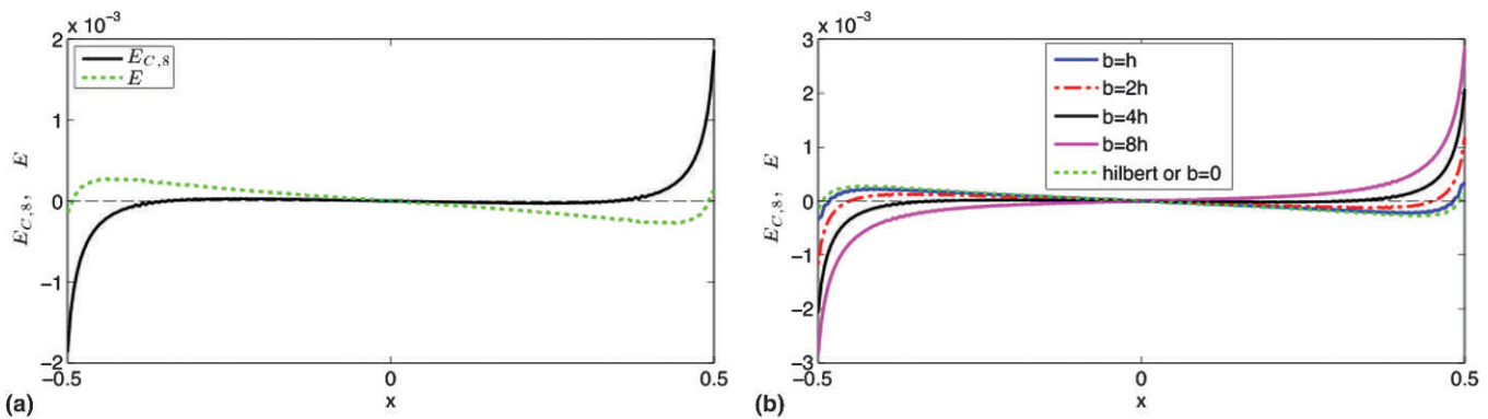
Fig. 9. (a) Error E_{C,8} of approximation of \text{Im}H(x) by -H[C_8(\text{Re}H(x))] with a periodic 8th degree polynomial continuation, N = 100 , b = 0.0202 compared with the error E with H[\text{Re}H(x)] without periodic continuation in the example of a finite element model of a DRAM package. (b) Errors E_{C,8} and E for various length of the extended domain: b = 0 (no continuation), b = h , 2h , 4h , and 8h , where h = 0.0051 .
