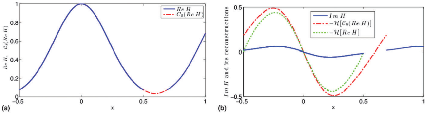
Fig. 12. (a) ReH(x) and C_8(ReH) in the delayed Gaussian example with t_d = 0.1 , N = 1001 , and b = 0.096 shown on [-0.51] . (b) ImH(x) and its reconstructions -\mathcal{H}[C_8(ReH)] and -\mathcal{H}[ReH] with and without continuations, respectively.
