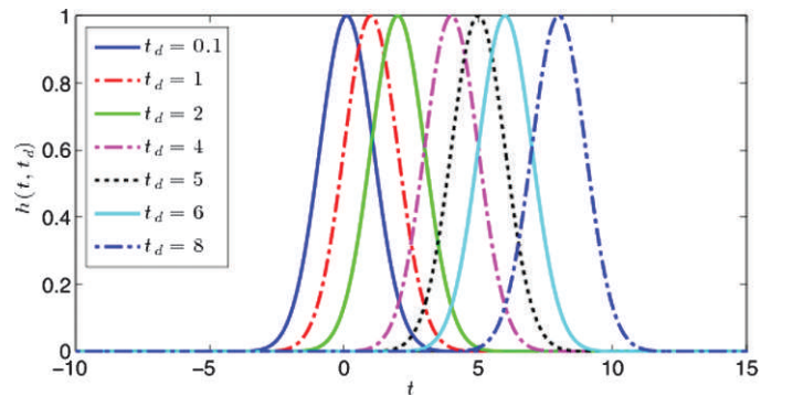
Fig. 11. Impulse-response function h(t, t_d) in the delayed Gaussian example with t_d varying from 0.1 to 8.
