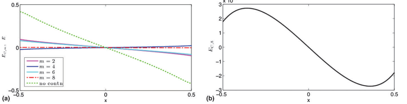
Fig. 3. (a) Errors E_{C,m} in reconstruction of ImH in the four-pole example using continuation C_m(ReH)(x) with polynomials of degree m = 2, 4, 6, 8 , and b = 1 , and E from the direct computation of Hilbert transform (without continuation) using Matlab function hilbert . (b) Zoom-in of the error E_{C,8}(x) .
